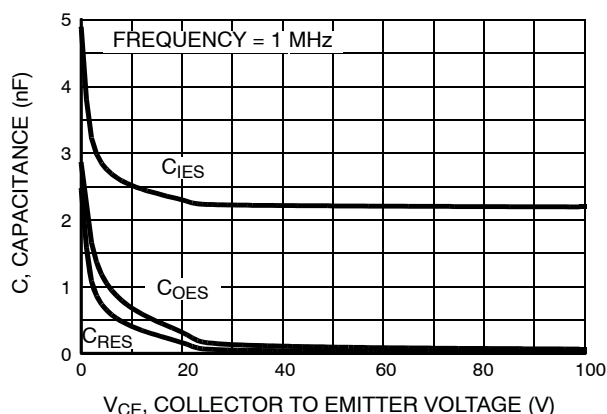
Figure 17. CAPACITANCE vs. COLLECTOR TO EMITTER VOLTAGE
