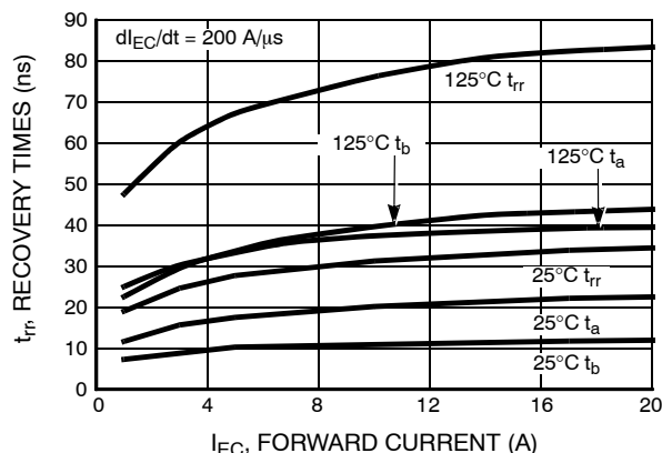
Figure 20. RECOVERY TIMES vs. FORWARD CURRENT
